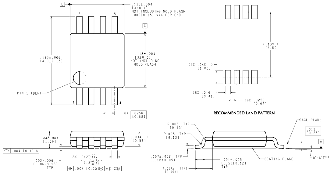
8-Lead MSOP Order Number DAC101S101CIMM NS Package Number MUA08A
