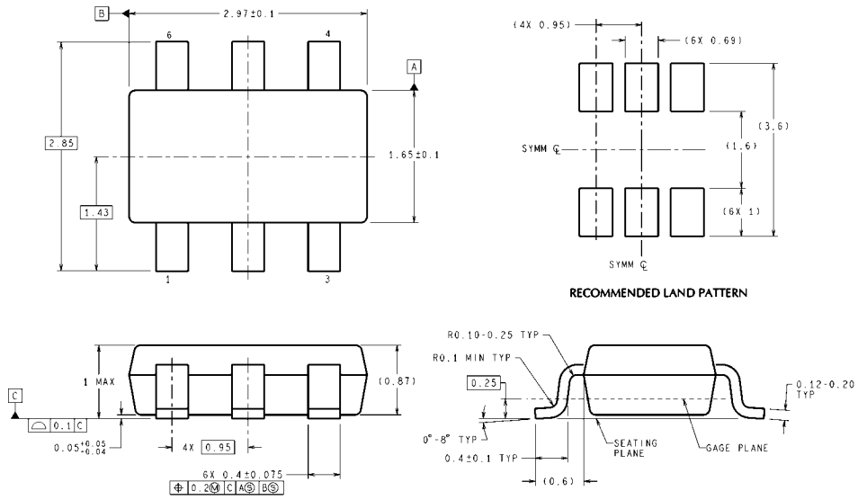
6-Lead TSOT Order Numbers DAC101S101CIMK and DAC101S101QCMK NS Package Number MK06A
